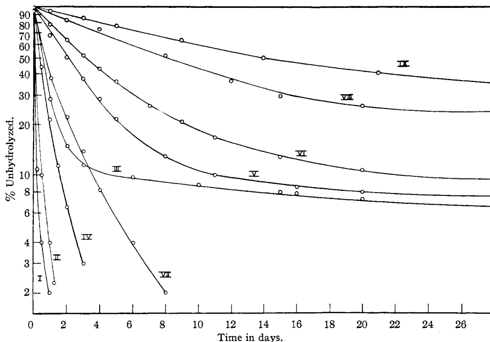
Fig. 1.—Rate of hydrolysis of unsymmetrical tetraalkyl pyrophosphates (RO)_2-POP(OR')_2 at 25^\circ ; 0.02 M solution: I, R = CH_3 , R' = C_2H_5 ; II, R = CH_3 , R' = n-C_3H_7 ; III, R = CH_3 , R' = i-C_3H_7 ; IV, R = C_2H_5 , R' = n-C_3H_7 ; V, R = C_2H_5 , R' = i-C_3H_7 ; VI, R = n-C_3H_7 , R' = i-C_3H_7 . 0.02 M in contact with water: VII, R = C_2H_5 , R' = n-C_4H_9 ; VIII, R = i-C_3H_7 , R' = n-C_4H_9 . IX, R = i-C_3H_7 , R' = i-C_3H_7 (tetra-isopropyl compound).
